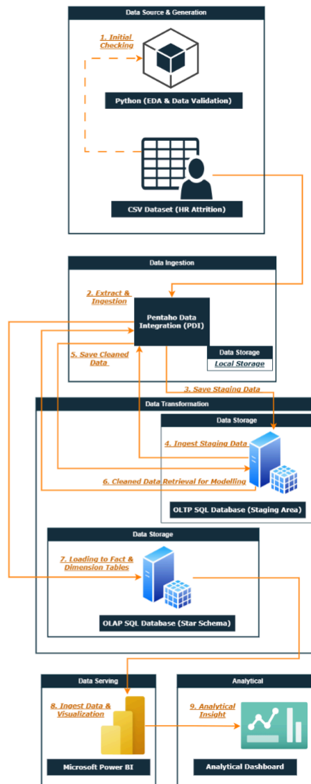
Fig. 4. Flowchart Research Framework
