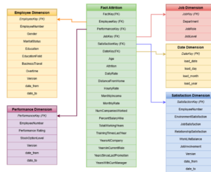
Fig. 9. Star Schema Dimensional Modelling
